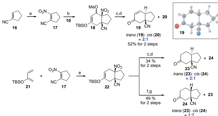
Scheme 2. Reagents and conditions: (a) \text{NaNO}_2 , CAN, \text{CH}_3\text{CN} , rt, 24 h, 61%; (b) toluene, 100^\circ\text{C} , 10 h, 95%; (c) n\text{-Bu}_3\text{SnH} , AIBN, benzene, reflux, 2 h; (d) HF, \text{CH}_3\text{CN} , 1 h; (e) toluene, 100^\circ\text{C} , 36 h, 63%, p -directed/ m -directed = 4:1; (f) HF, \text{CH}_3\text{CN} , rt, 8 h; (g) n\text{-Bu}_3\text{SnH} , AIBN, benzene, reflux, 1.5 h, 48% for two steps.
